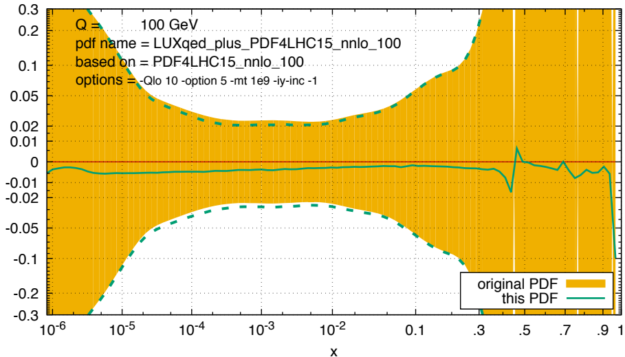
ratio of dbar to that in base (non-QED) set
