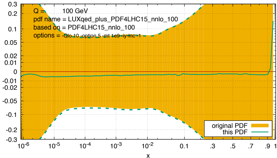
ratio of strange quark to that in base (non-QED) set
