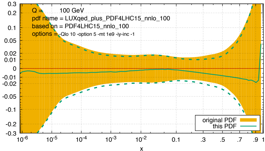
ratio of up quark to that in base (non-QED) set
