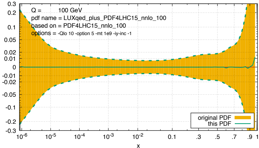
ratio of photon relative that in paper v1 (both via LHAPDF files)
