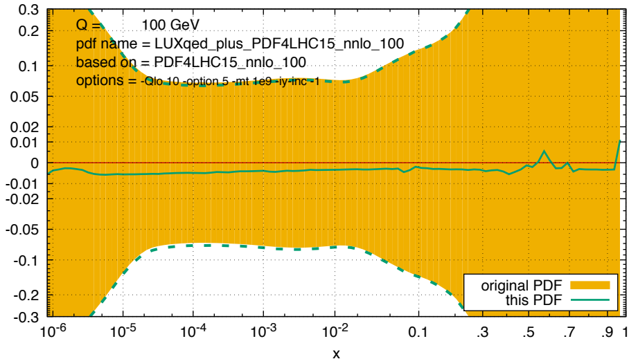
ratio of sbar to that in base (non-QED) set
