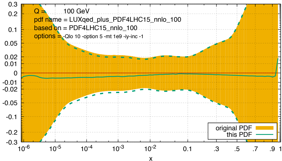
ratio of down quark to that in base (non-QED) set
