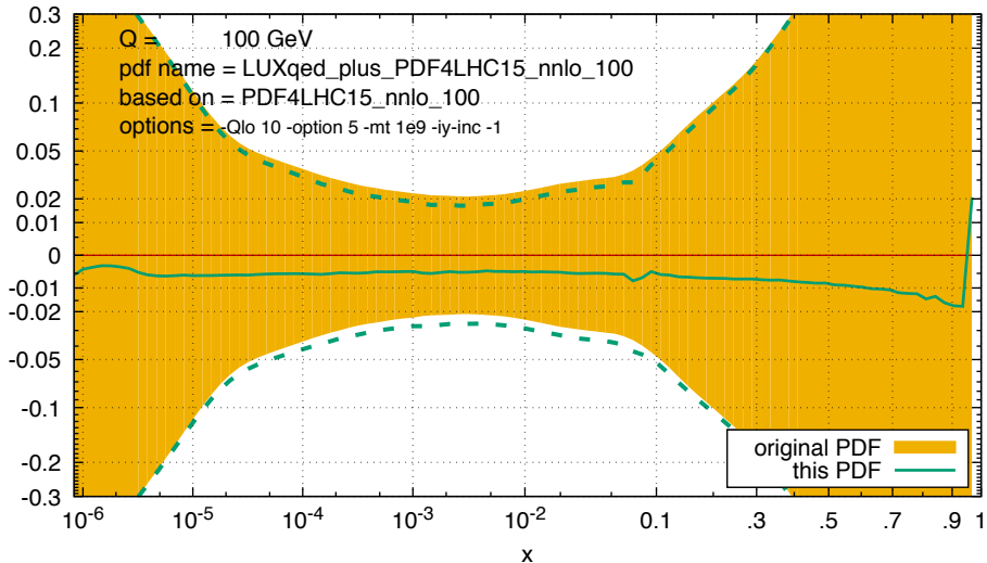
ratio of charm quark to that in base (non-QED) set
