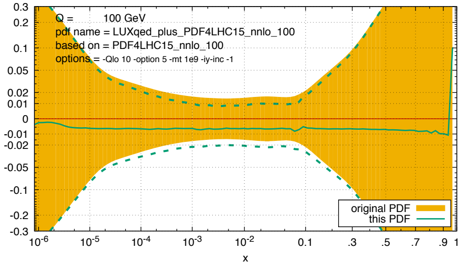
ratio of gluon to that in base (non-QED) set
