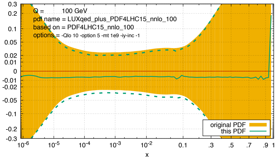
ratio of bottom quark to that in base (non-QED) set
