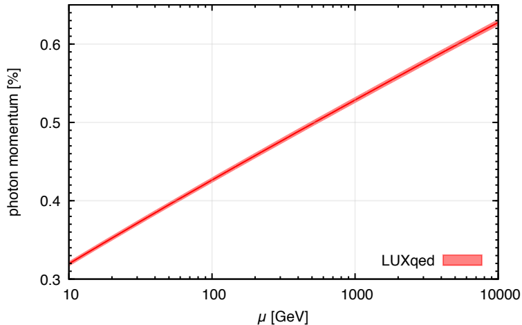
percentage of proton's momentum carried by photon
