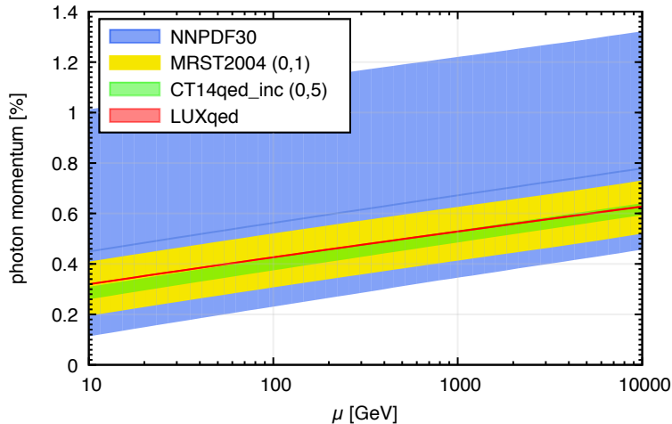
percentage of proton's momentum carried by photon
